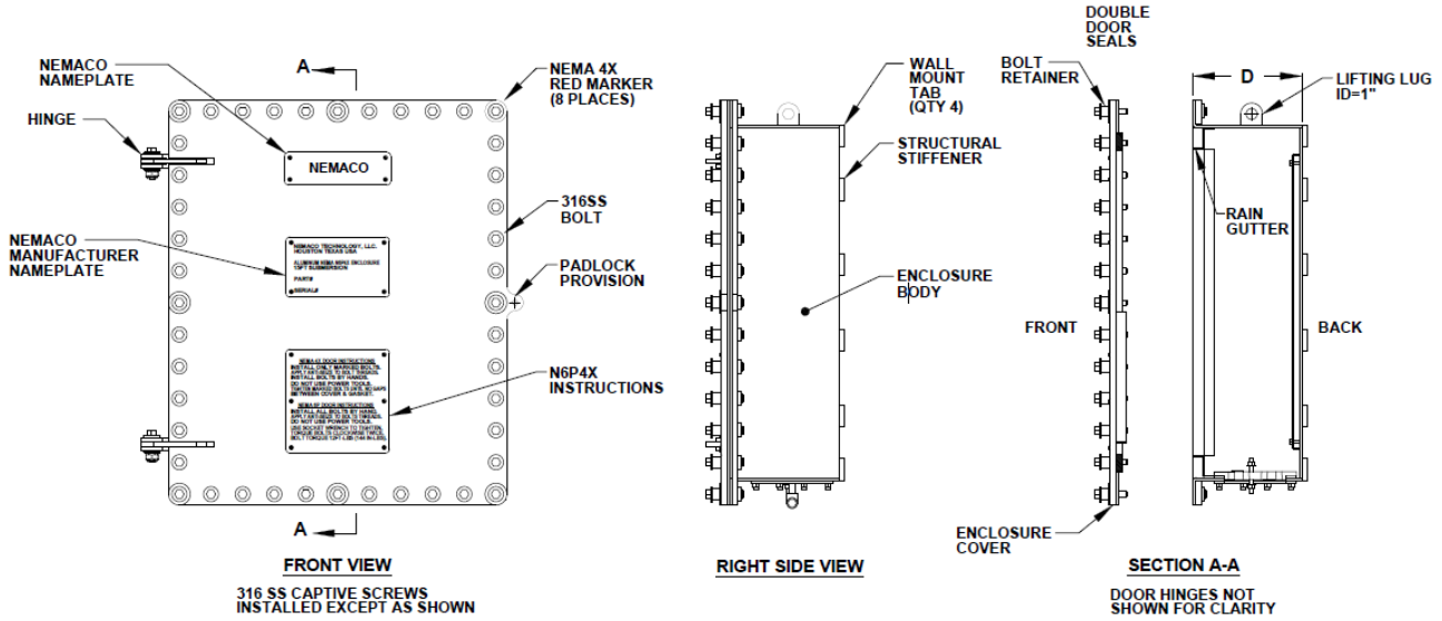
FIGURE 1 Nemaco Submersible N6P4X - Enclosure Door with Double Seals
