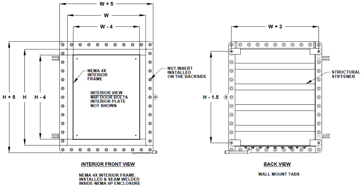
FIGURE 2 Nemaco Submersible N6P4X - Door Removed and Back Side View
