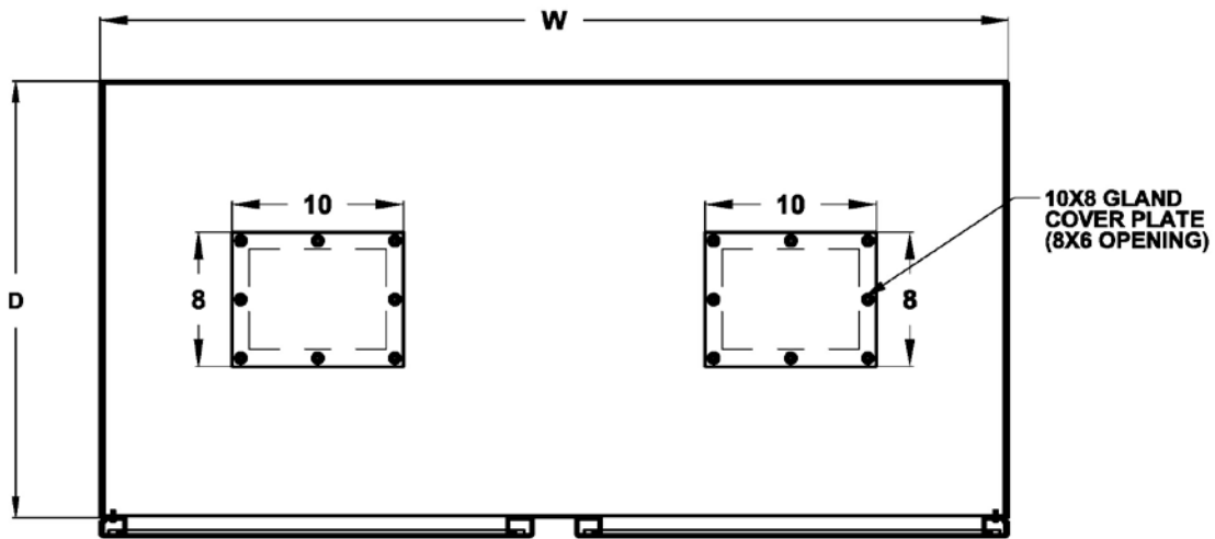
FIGURE 4 SECTION VIEW A-A COVER PLATE OPTIONS
