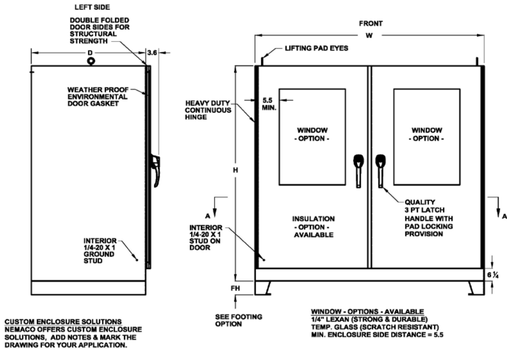
FIG. 1 - NEMA 4X - "PCE" STAINLESS STEEL ENCLOSURE - EXTERIOR DIMENSIONS
