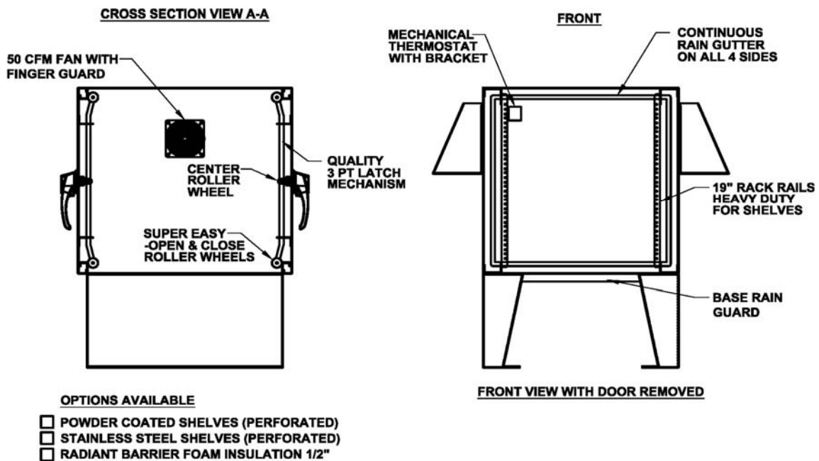
FIG. 2 - NEMA 3R - "PCE" STAINLESS STEEL ENCLOSURE - INTERIOR DIMENSIONS & HARDWARE
