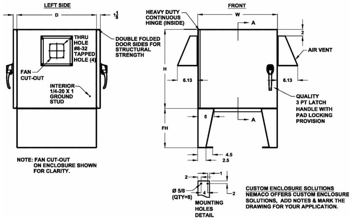
FIG. 1 - NEMA 3R - "PCE" STAINLESS STEEL ENCLOSURE - EXTERIOR DIMENSIONS
