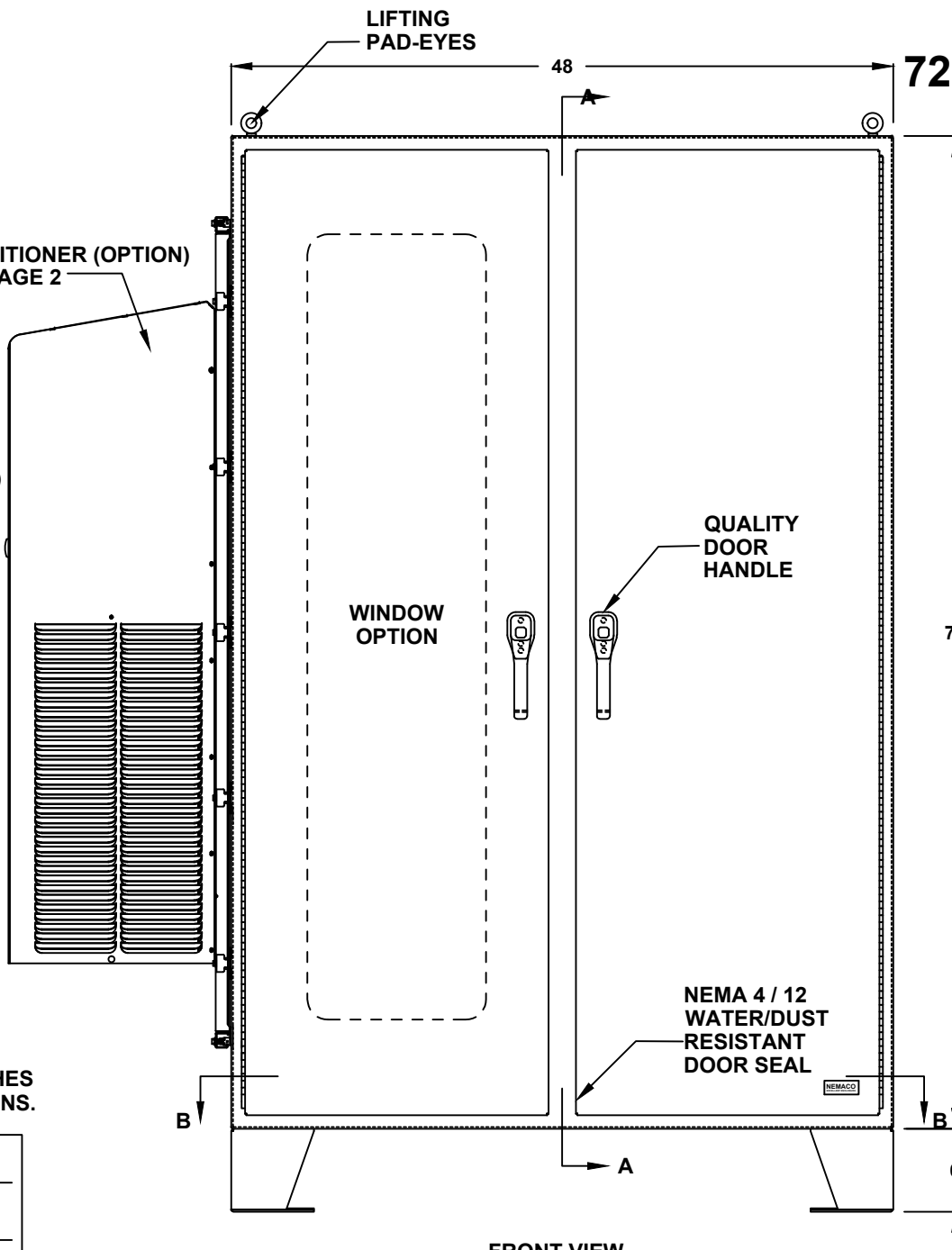
FRONT VIEW
