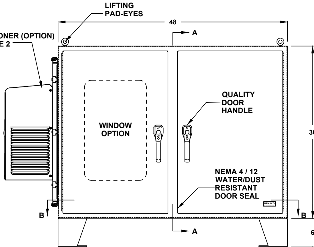
FRONT VIEW
