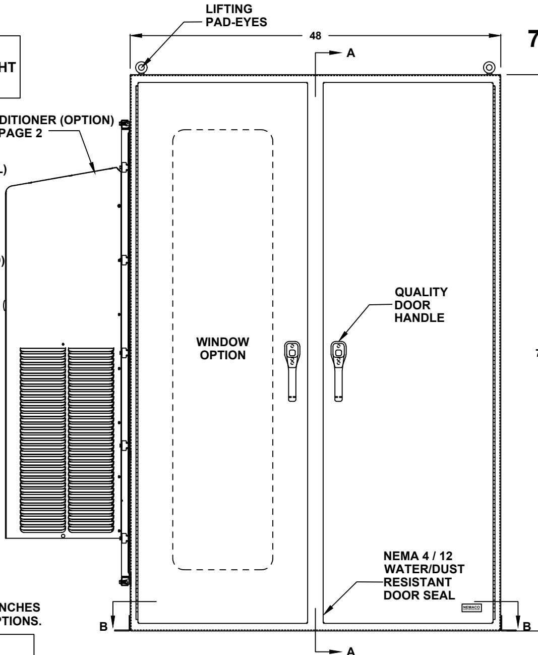
FRONT VIEW
