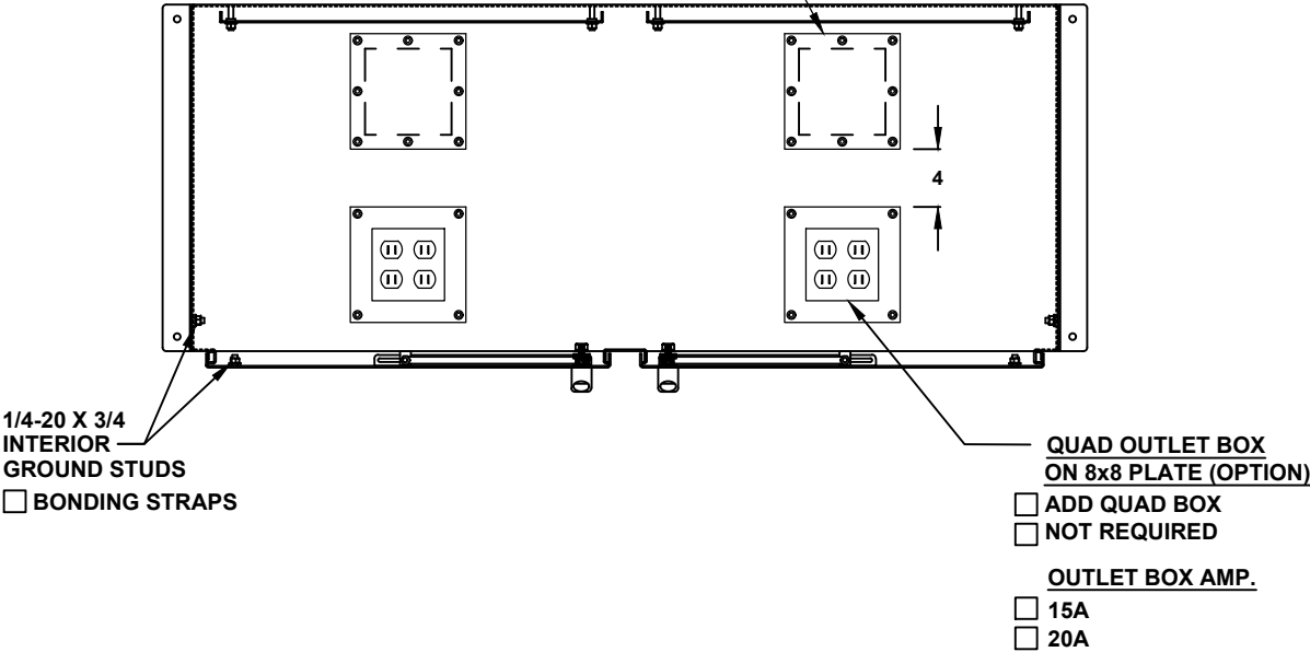
TOP CROSS SECTION VIEW B-B
