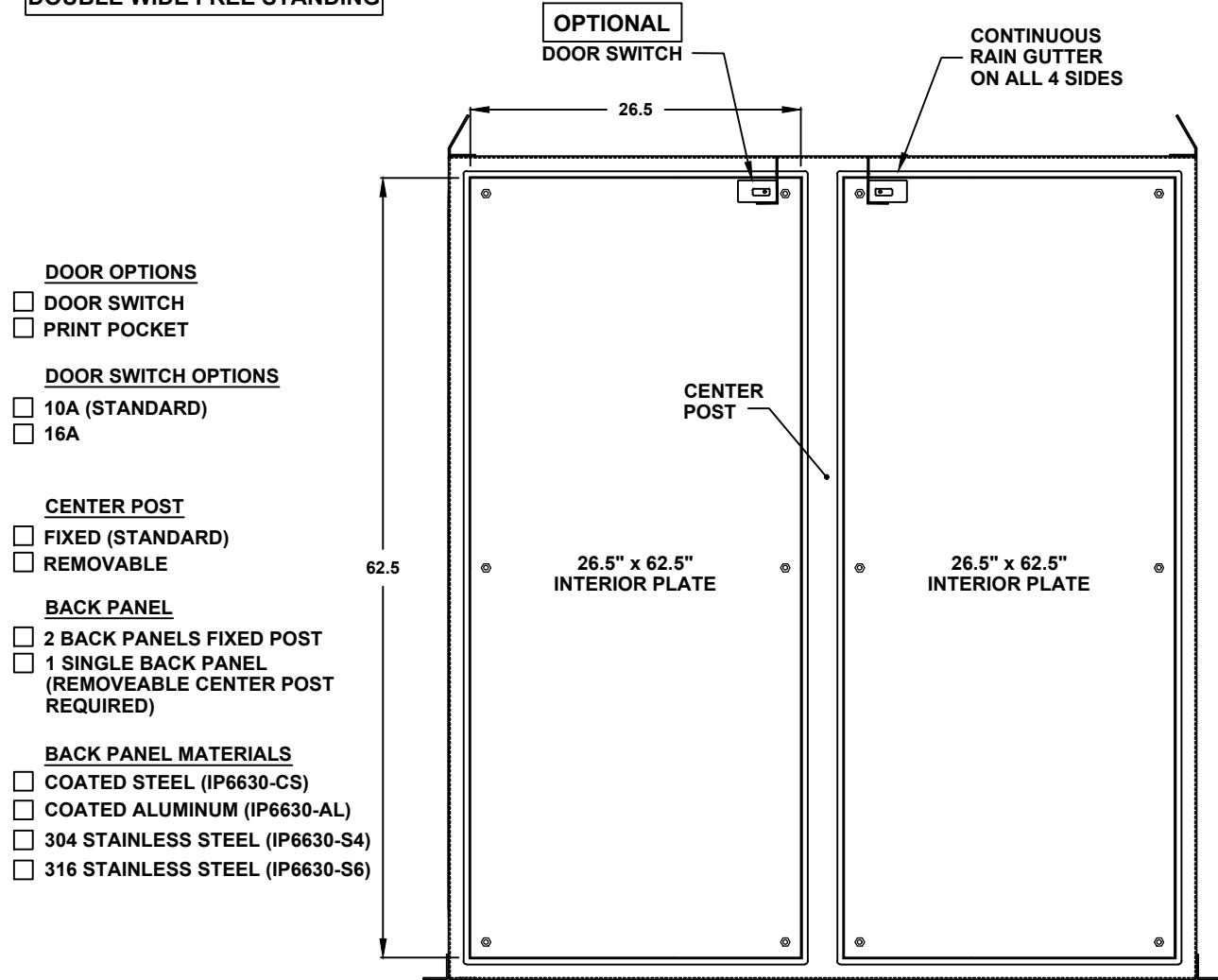
FRONT VIEW WITH DOOR REMOVED
