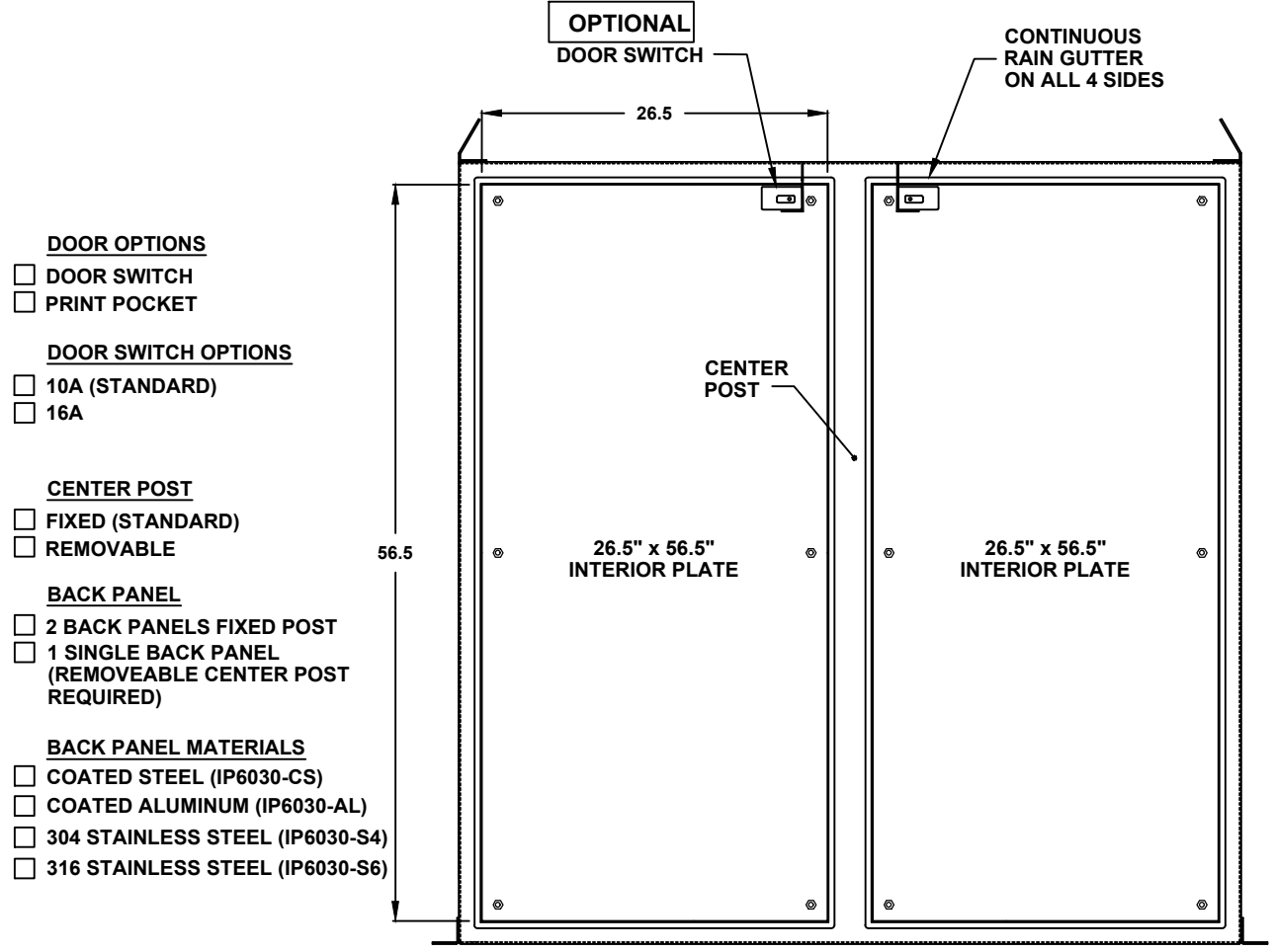
FRONT VIEW WITH DOOR REMOVED
