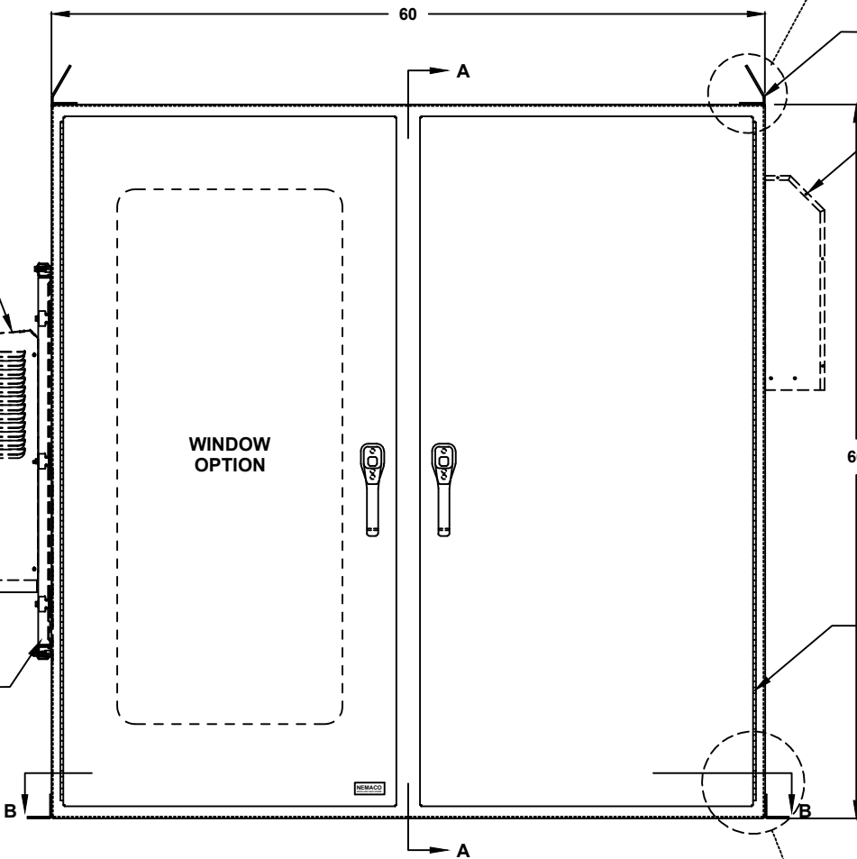
FRONT VIEW
