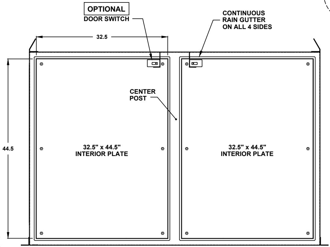
FRONT VIEW WITH DOOR REMOVED
