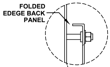
DETAIL C-C
