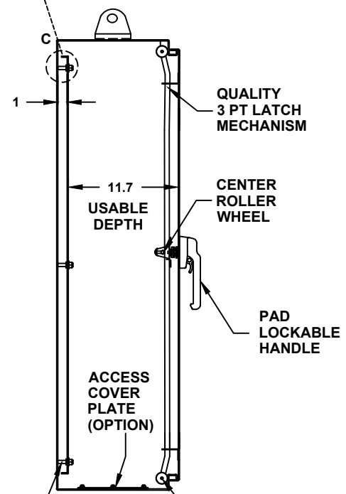
DETAIL C-C
