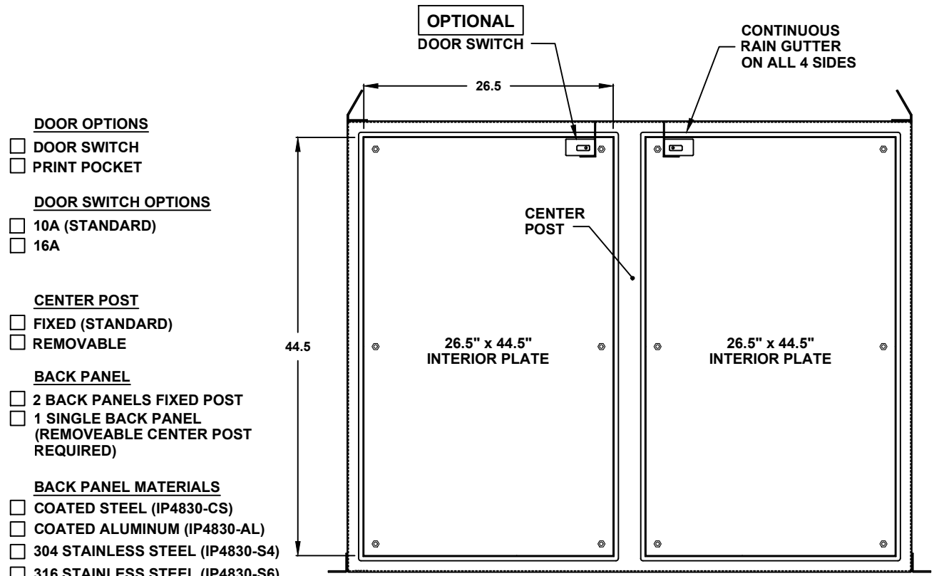
FRONT VIEW WITH DOOR REMOVED
