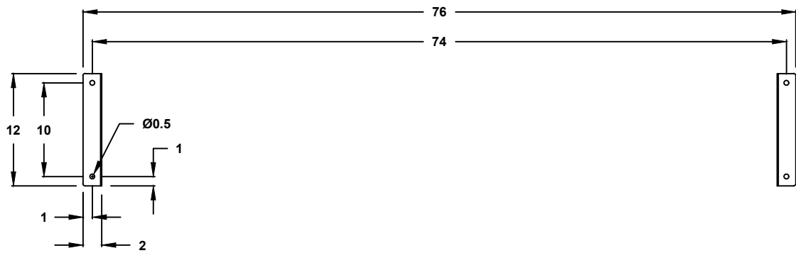
ENCLOSURE MOUNTING BRACKET DETAILS
