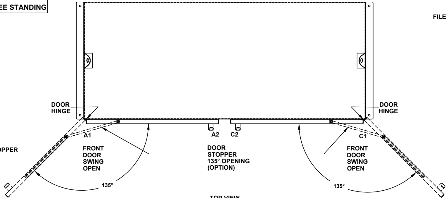
TOP VIEW
