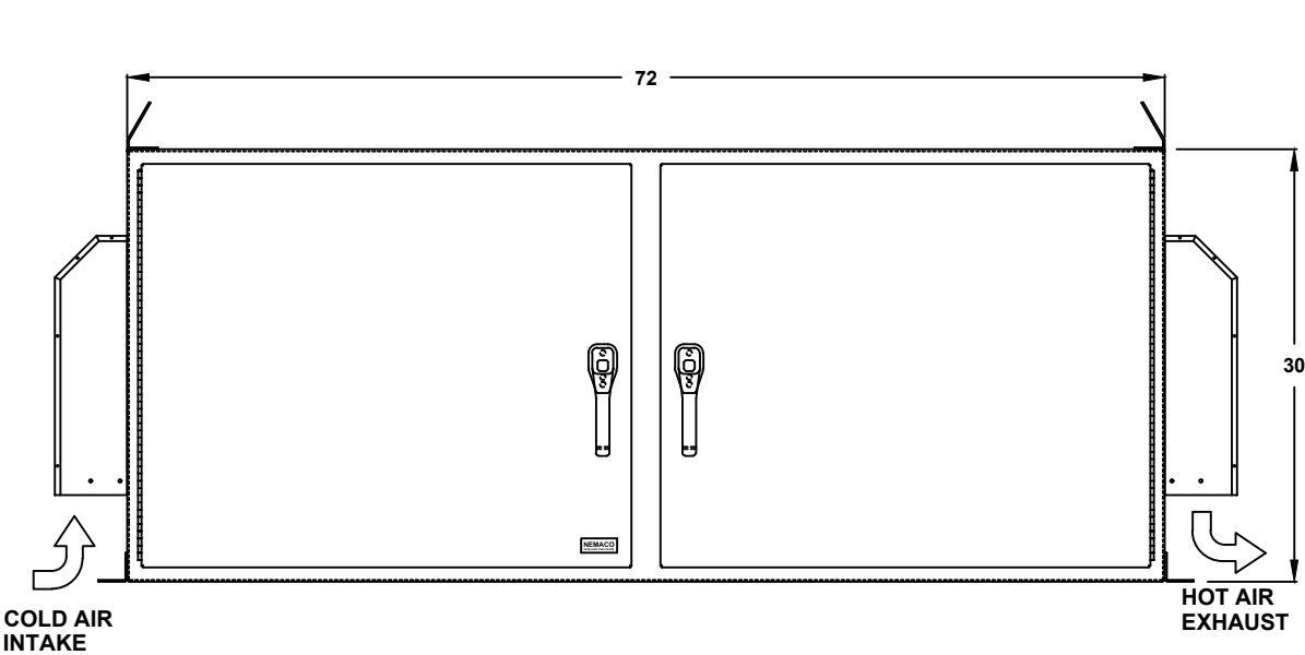
FRONT VIEW
