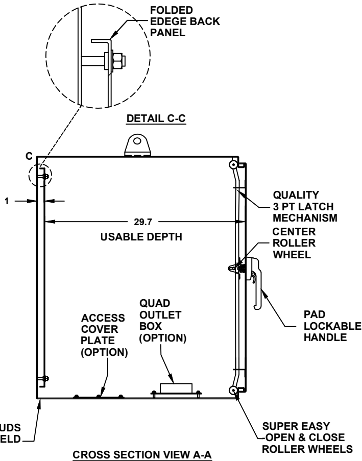
CROSS SECTION VIEW A-A
