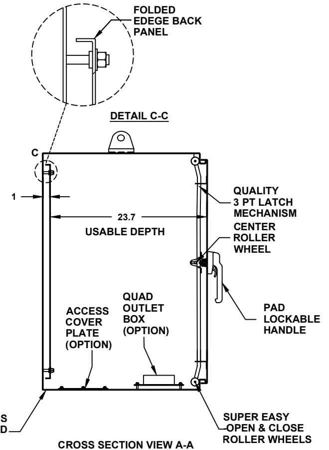
CROSS SECTION VIEW A-A
