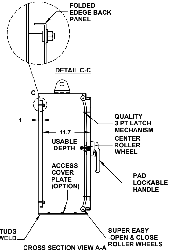
CROSS SECTION VIEW A-A
