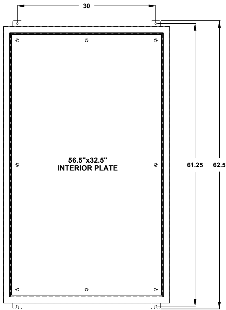
FRONT VIEW WITH DOOR REMOVED
