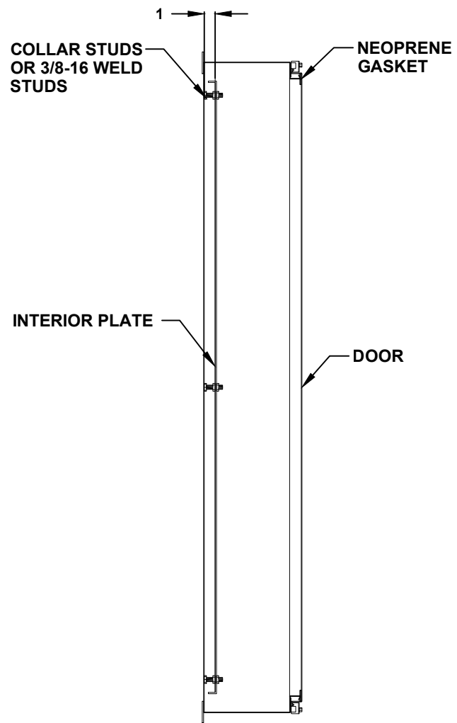
CROSS SECTION VIEW A-A
