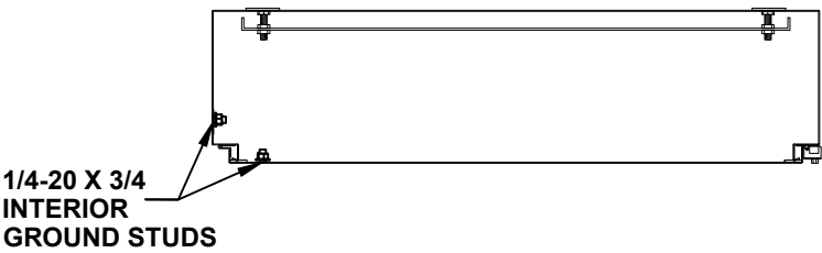
CROSS SECTION VIEW B-B
