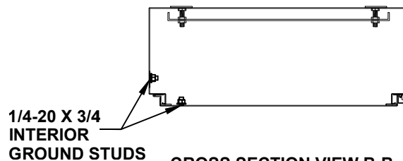
CROSS SECTION VIEW B-B
