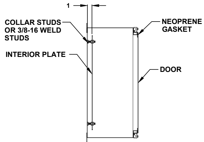
CROSS SECTION VIEW A-A
