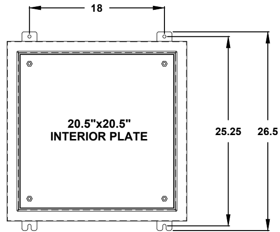
FRONT VIEW WITH DOOR REMOVED
