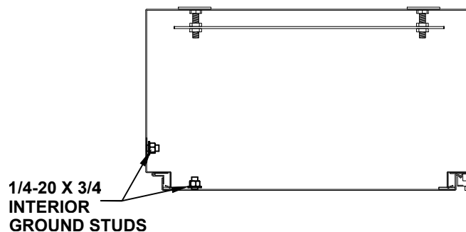
CROSS SECTION VIEW B-B
