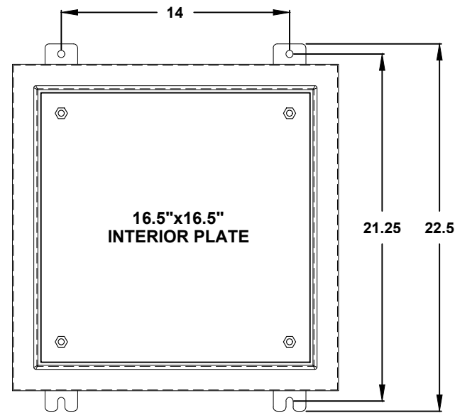
FRONT VIEW WITH DOOR REMOVED
