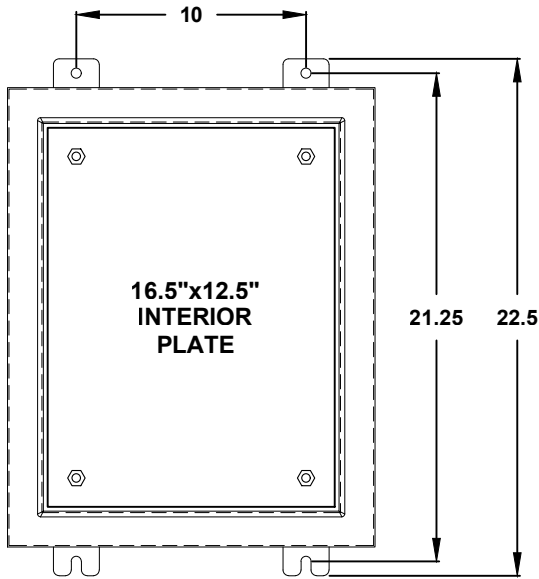
FRONT VIEW WITH DOOR REMOVED
