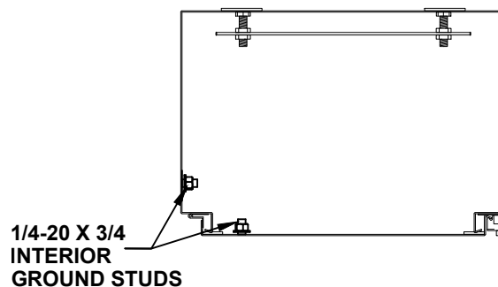
CROSS SECTION VIEW B-B
