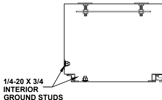
CROSS SECTION VIEW B-B
