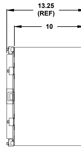
RIGHT VIEW
