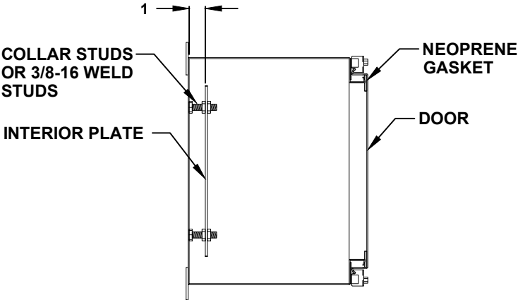
CROSS SECTION VIEW A-A
