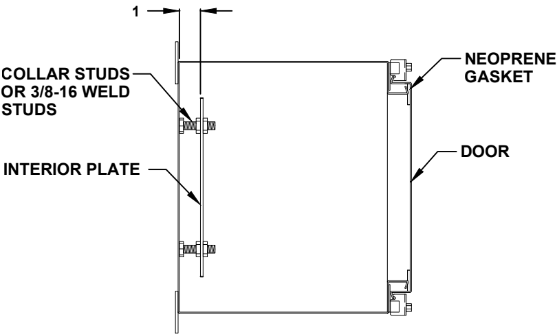
CROSS SECTION VIEW A-A
