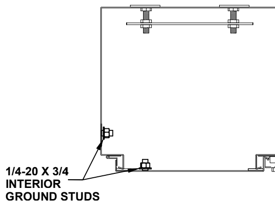
CROSS SECTION VIEW B-B
