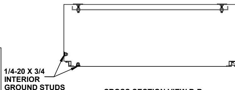
CROSS SECTION VIEW B-B
