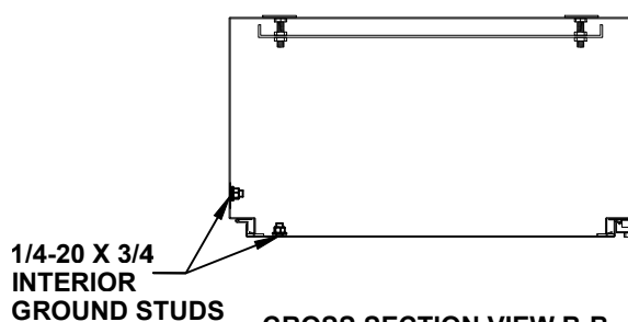
CROSS SECTION VIEW B-B
