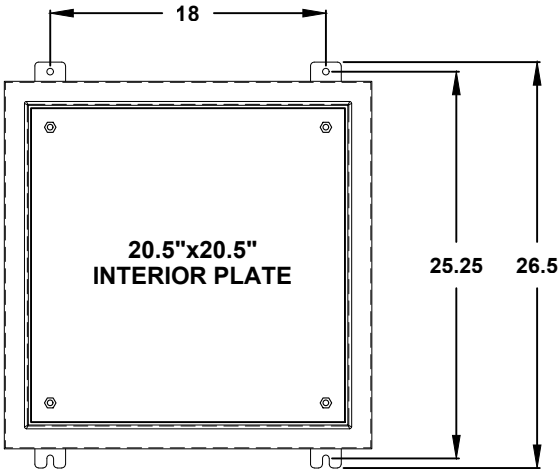
FRONT VIEW WITH DOOR REMOVED
