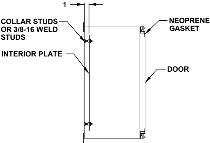
CROSS SECTION VIEW A-A
