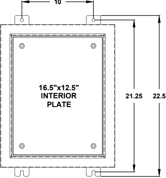
FRONT VIEW WITH DOOR REMOVED
