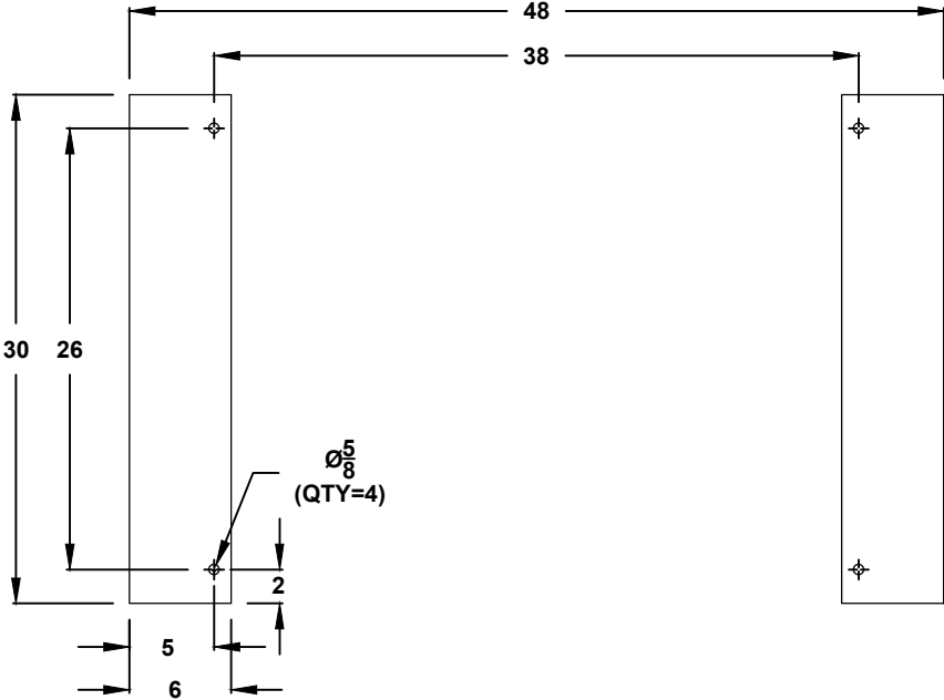
CROSS SECTION VIEW C-C MOUNTING HOLES
