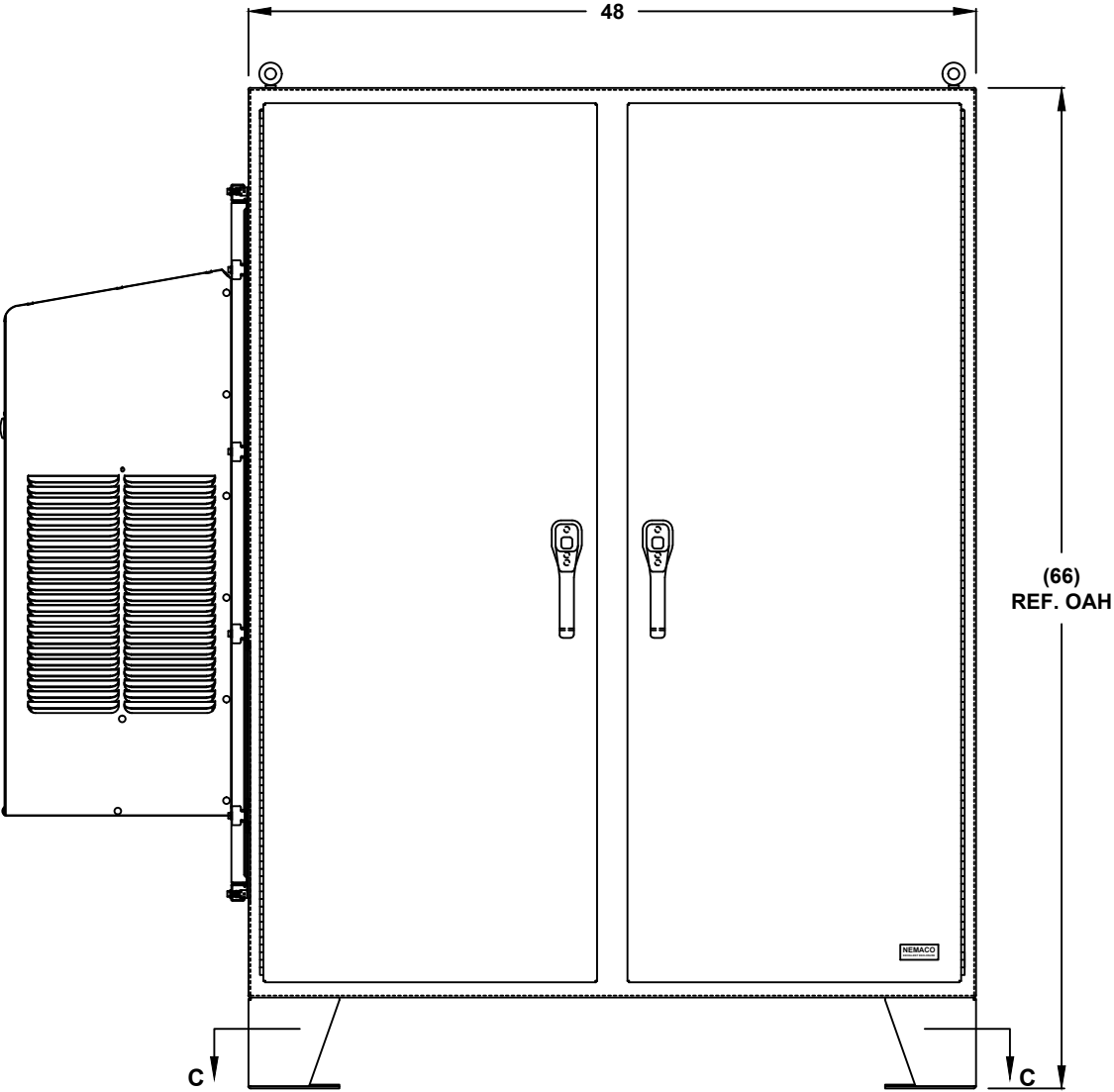
FRONT VIEW
