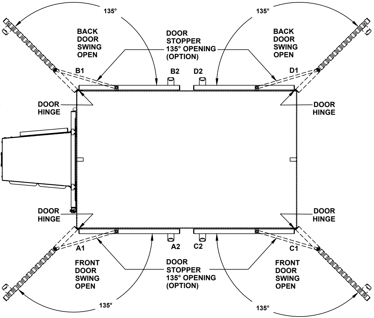
TOP VIEW
