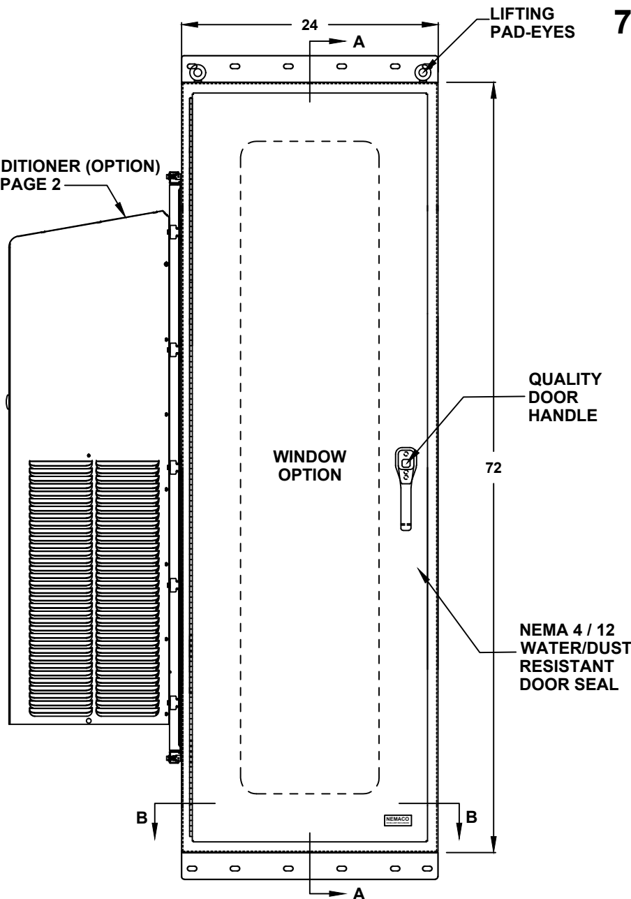
FRONT VIEW
