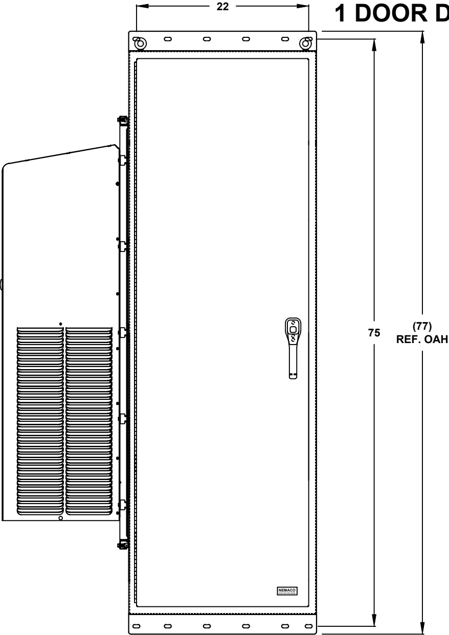
FRONT VIEW
