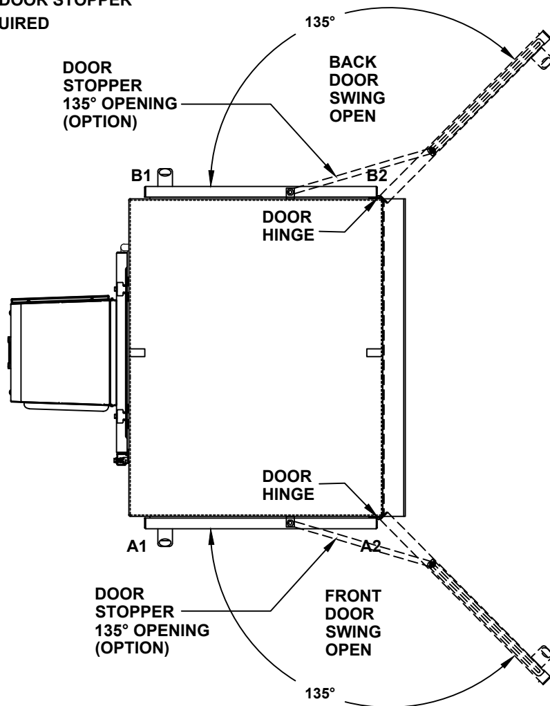
TOP VIEW
