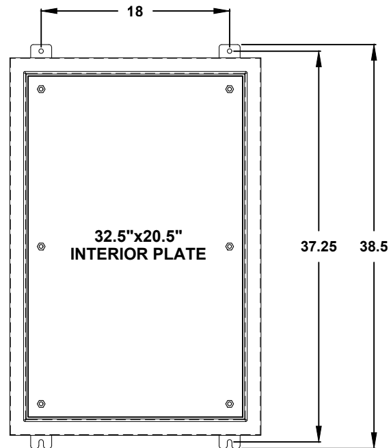
FRONT VIEW WITH DOOR REMOVED
