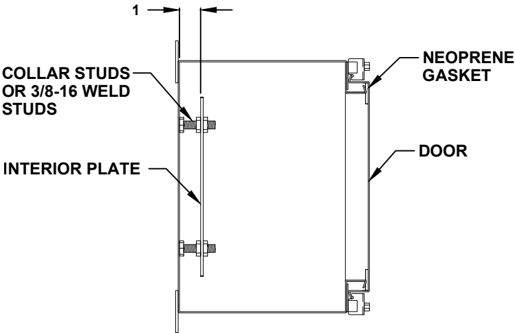
CROSS SECTION VIEW A-A
