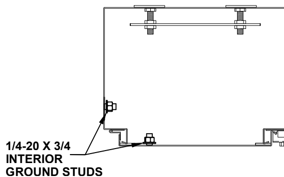
CROSS SECTION VIEW B-B
