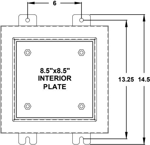
FRONT VIEW WITH DOOR REMOVED
